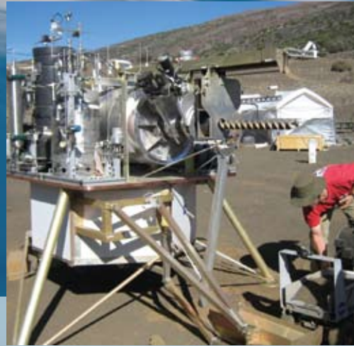
Prototype lunar oxygen production system
